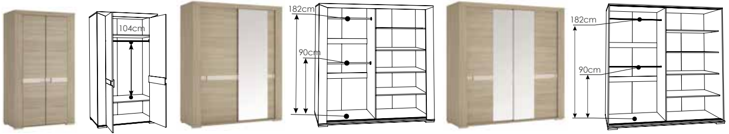
type 20 →/↑/↗ 109/192/57,5cm
