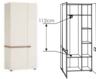
type 25 →/↑/↗ 84,9/194,5/36,9cm
