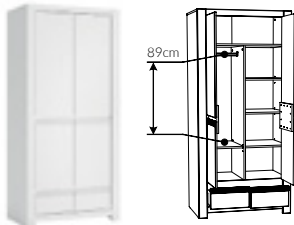
type NVIS02 →/↗ 92/198,5/58,2cm
