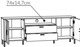
type SHIV101 →/↑/↗ 82,1/156/40cm Square 1 point – optional lighting
