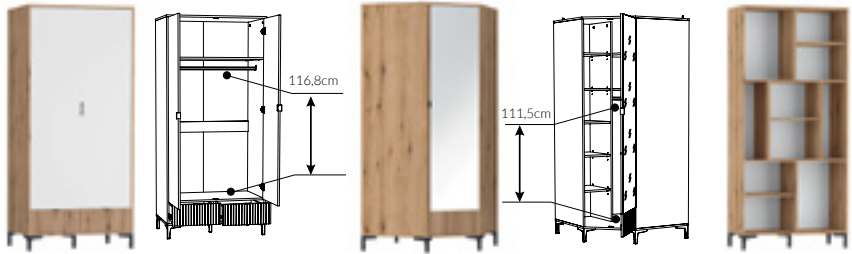
type RIKS01 →/↑/↗ 91,5/198/56cm type RIKS02 ←→ →/↑/↗ 90/198/90cm type RIKR01 →/↑/↗ 91,5/198/40cm
