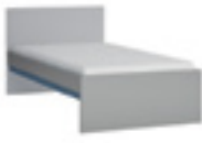
type LASZ01 →/↑/↗ 96/80,5/206,1cm optional products (sold separately): - MWSD01 flexible frame, - 90x200cm main mattress (Impresso MWMP06, Elio MWMP04) - additional mattress 80x190 max. height 15cm (Tukan MWMU03) - drawer with additional sleeping function LASZ02
