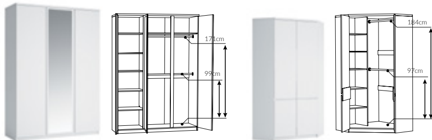
type FRIS03 →/↗/↘ 155,3/220/58cm type FRIS05 →/↗/↘ 95/200/95cm
