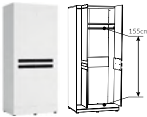
type VISS01 →/↑/↗ 86/200/58,6cm
